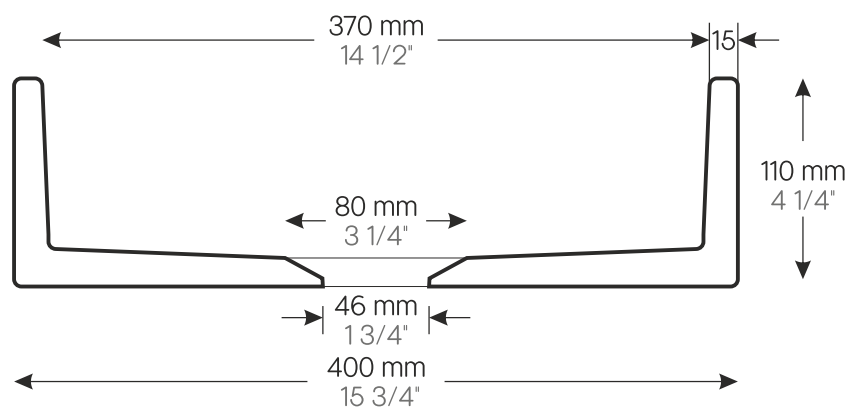
SECTION VIEW
