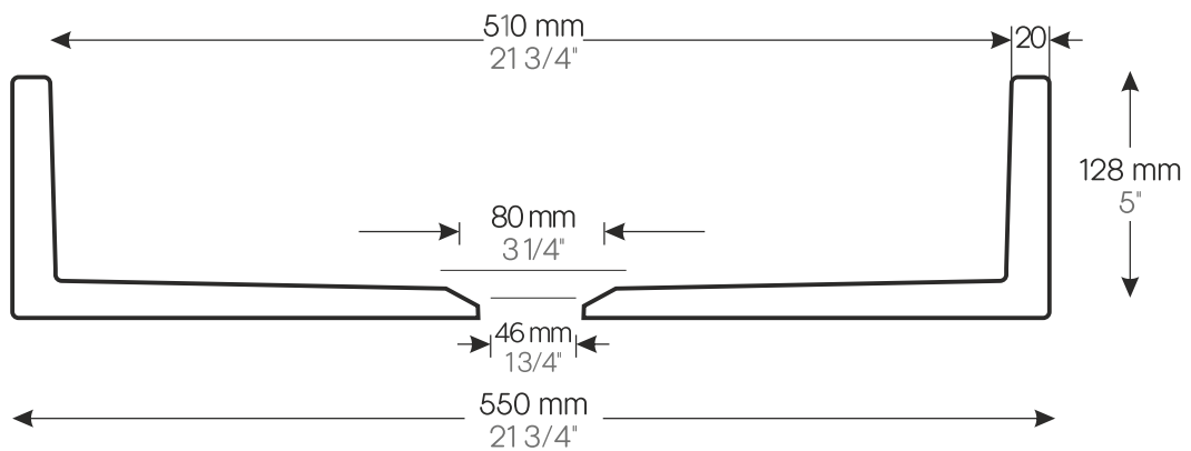
SECTION VIEW
