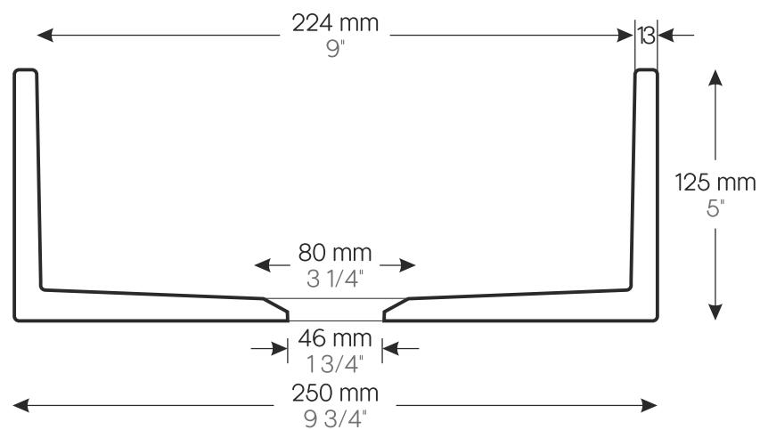
SECTION VIEW
